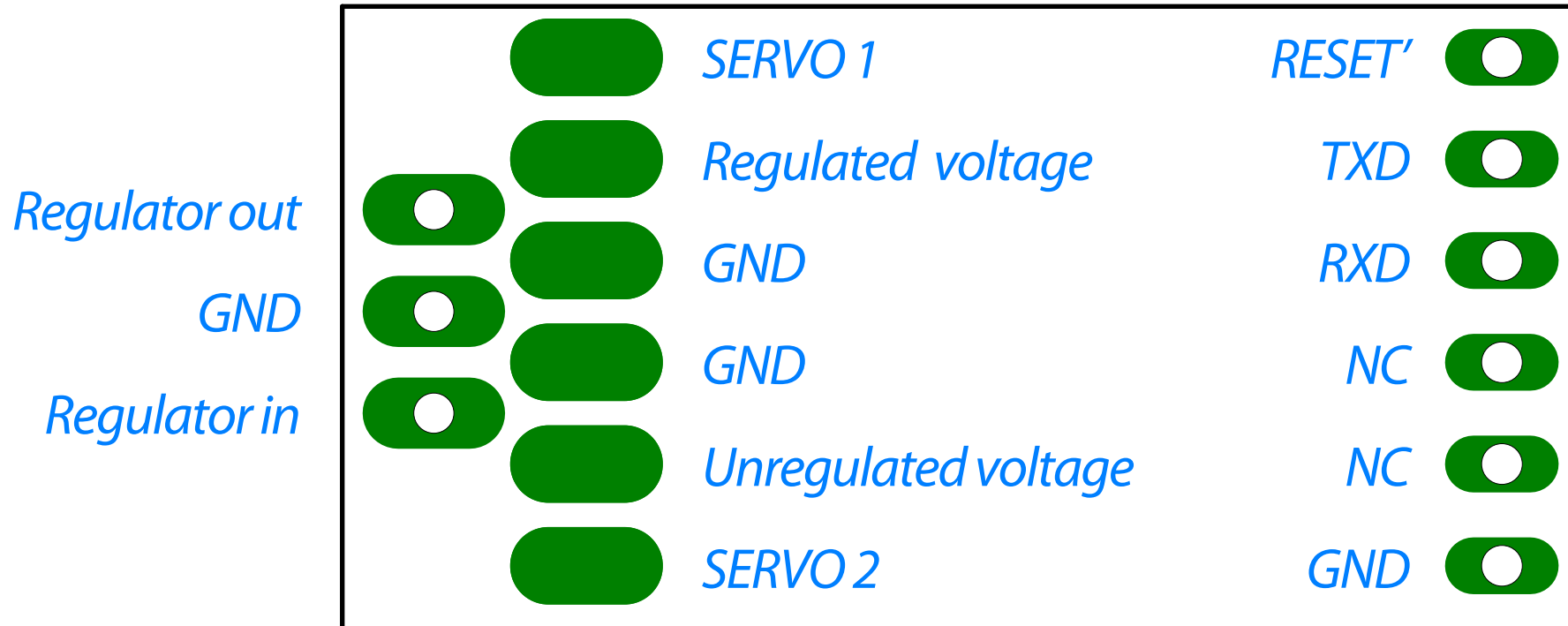
Bottom view (side with ATmega328P)
